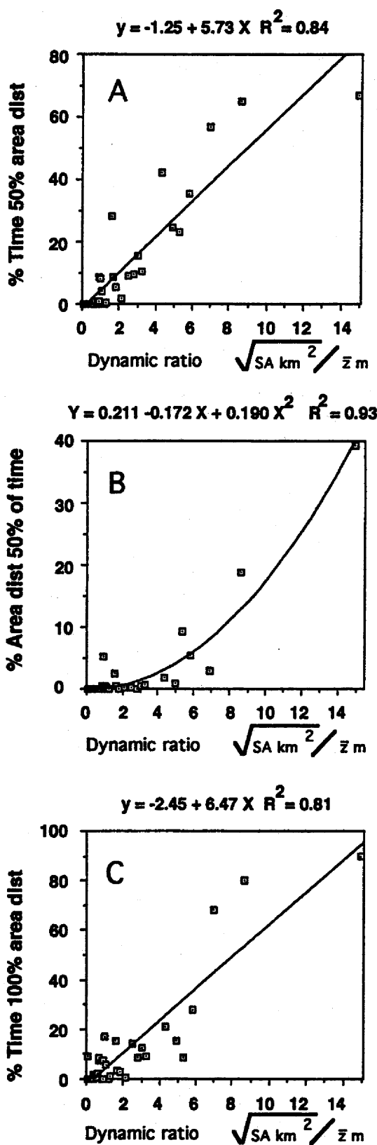
Figure 4.—Best fit analysis of the per cent of the time that 50% of the lakebed is disturbed, per cent of the time that 100% of the lakebed is disturbed, and the per cent of the lake area that is disturbed 50% of the time versus the dynamic ratio for the 36 lakes in this study.
