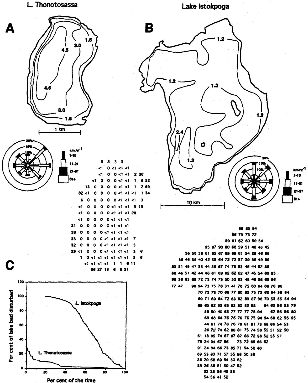
Figure 1.-A. Contour map and wind rose for Lake Thonotosassa and calculated per cent of the time that waves are expected to disturb the sediments at each of the grid intersections. Values listed as <1 are disturbed less than 1 but more than 0% of the time. B. Similar maps for Lake Istokpoga. C. The per cent of the lakebed subject to wave disturbance for different percentages of time for Lake Thonotosassa and Lake Istokpoga.
